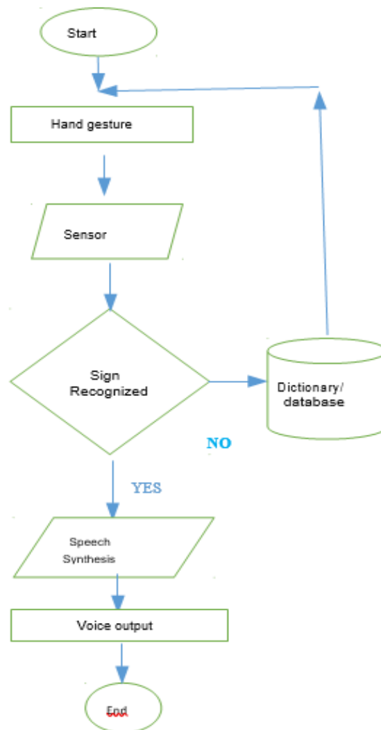
FIG 4.2 SYSTEM FLOWCHART
